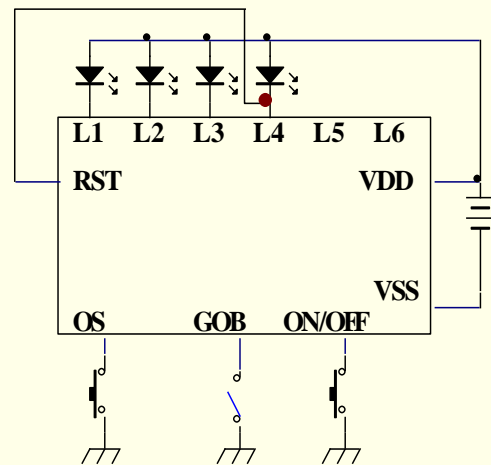
Example 9: Apply RST key as 4LED control with external resistance
