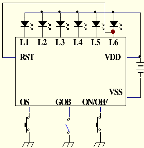
Example 8: Apply RST key as 4LED control without external resistance .
