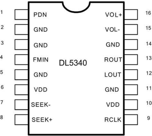
Figure 3-1. DL5340 Top View
