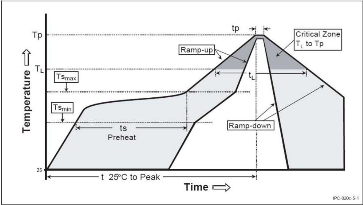
Figure 5-4.Classification Reflow Profile
