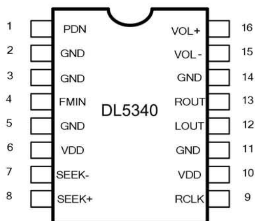
Figure 1-1. DL5340 Top View
